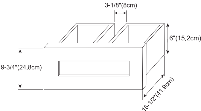
FRONT DRAWER VIEW
