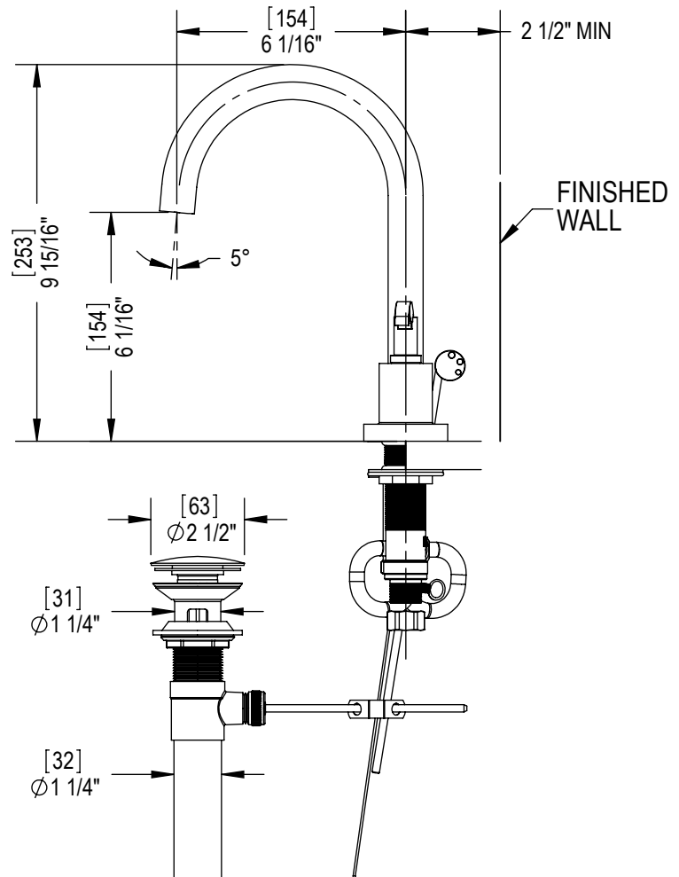
Critical Dimensions
