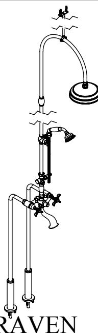
Floor Mount Tub & Shower w ith Optional Hand Held Shower Model: 2FRBRVC XX-XX
