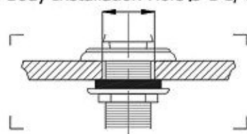
Body Installation Hole Ø 1 1/4"
