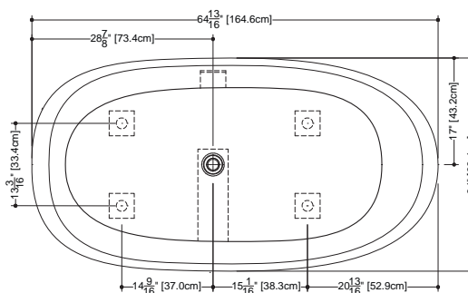
plan view
