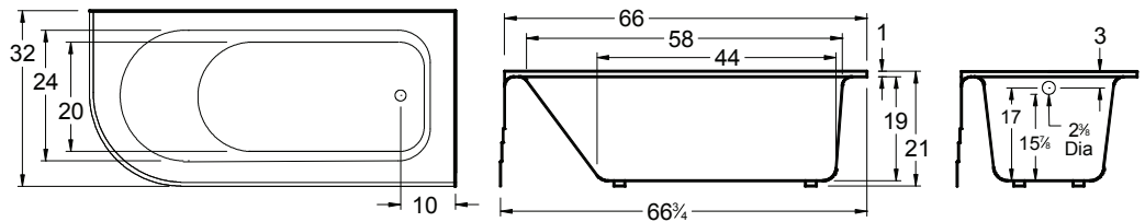
Tub pictured with optional waste & overflow.
