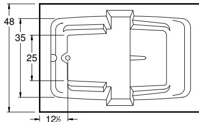
Tub pictured with optional waste & overflow
