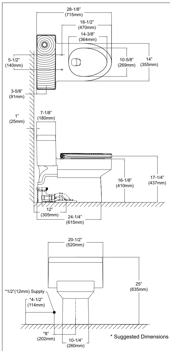
MS984244CFG - Ryohan Universal Height, One-Piece Toilet
