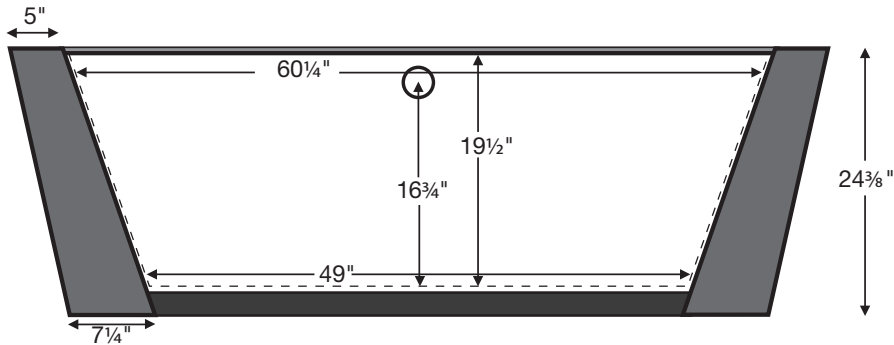
Dimensions for Eryx Wall-Mount with System Aria and pedestal base. Soaker dimensions are on the front of this specification sheet.
