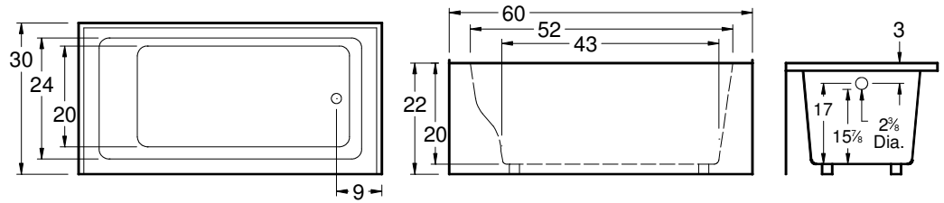
Tub pictured with optional waste &amp; overflow.
