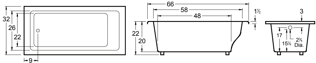
Tub pictured with optional waste & overflow.
