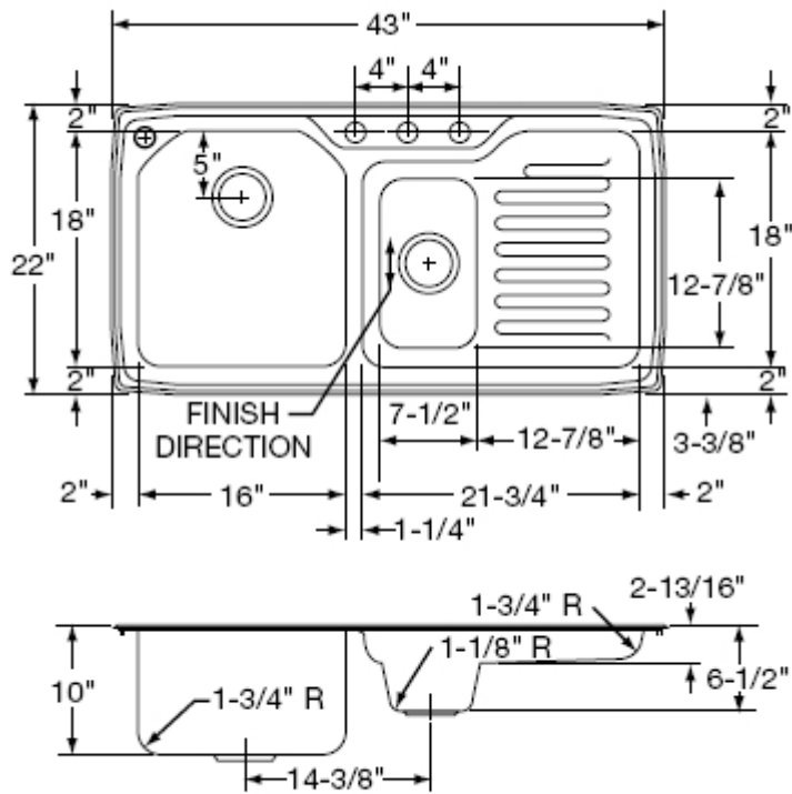
Model EGPI4322L4 Illustrated
