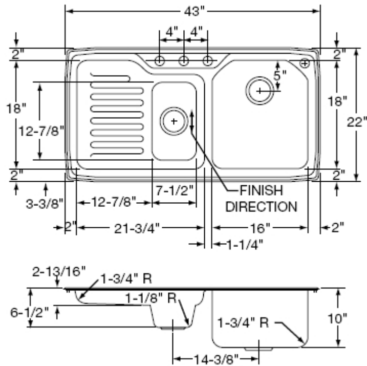
Model EGPI4322R4 Illustrated
