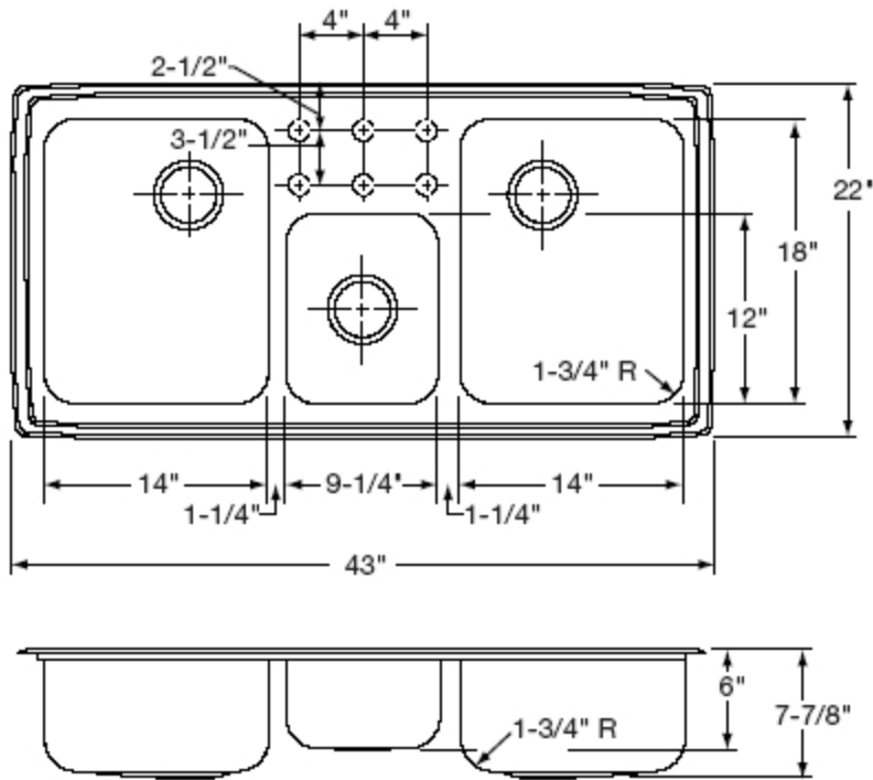
Model LCR43226 Illustrated
