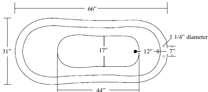
Rough-In Plumbing Measurements
