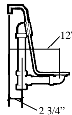
Rough-In Plumbing Measurements
