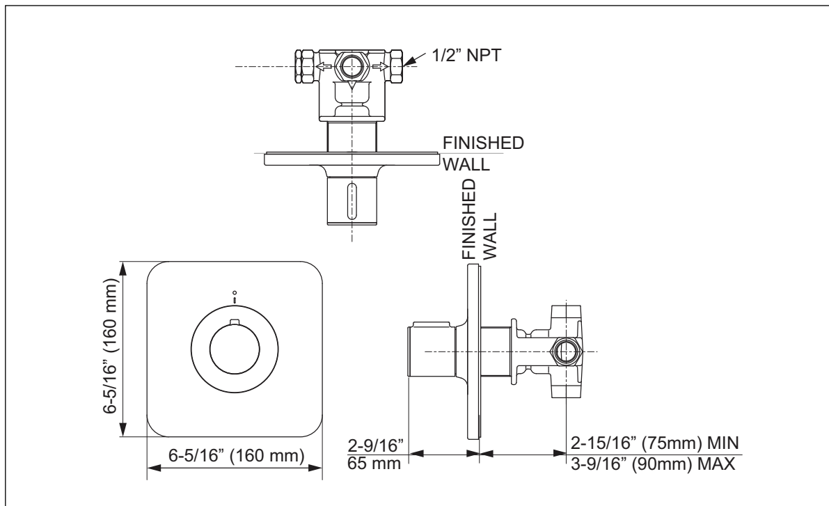
TS170C1 - Kiwami™ Renesse® Single Volume Control for Hand Shower (trim)
