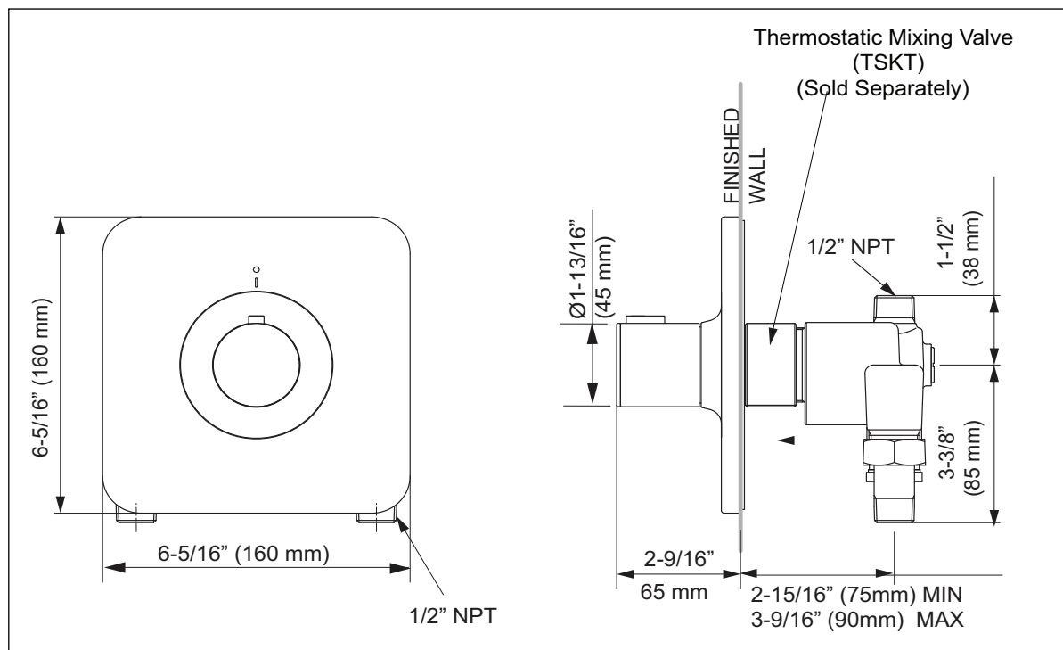
TS170T#CP - Kiwami™ Renesse® Thermostatic Mixing Valve (trim)
